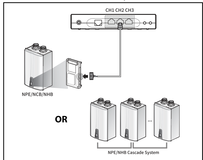
Installation Example
