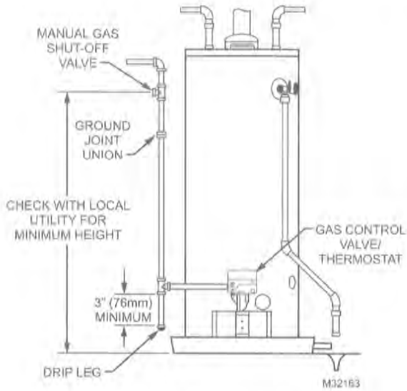
Fig. 1. Gas Piping.
